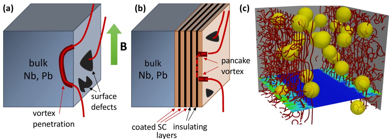
FIG. 8. Surface disorder and multilayers in SRF cavities. (a) Sketch showing how vortices (red) parallel to the surface of a cavity wall penetrate the wall (outside the superconductor, the red lines illustrate field lines), (b) intercalating insulating layers (S|I|S) will cause vortex pancakes to form and might limit the penetration depth of vortices. 231,232 (c) Simulation snapshot of surface vortex penetration into a type-II superconductor having spherical defects (yellow) near the surface in an AC magnetic field parallel to the surface. Vortex lines are shown in red. The planar projection shows the superconducting order parameter amplitude.
